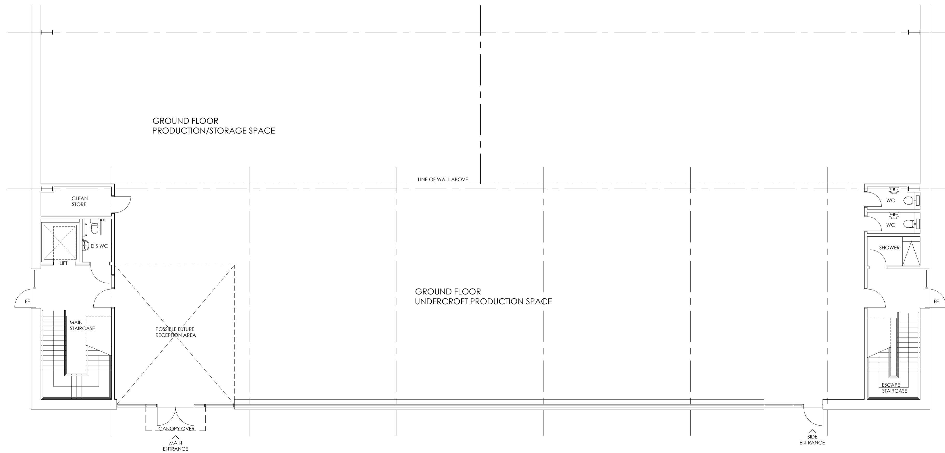
GROUND FLOOR PLAN SHOWING ENTRANCE AREA
